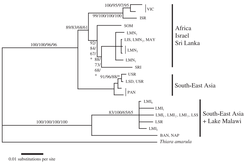
Fig. 3 Phylogenetic tree based on partial CO1 sequences of Melanoides tuberculata morphs with the outgroup Thiara amarula . Tree constructed using the neighbour-joining method on uncorrected P -distances. Numbers on branches represent Bayesian posterior probabilities, followed by maximum parsimony, maximum likelihood and minimum evolution bootstrap percentage support, respectively. Only values greater than 50% are shown, * indicates support less than 50% in minimum evolution analysis. For codes see legend to Fig. 1.
